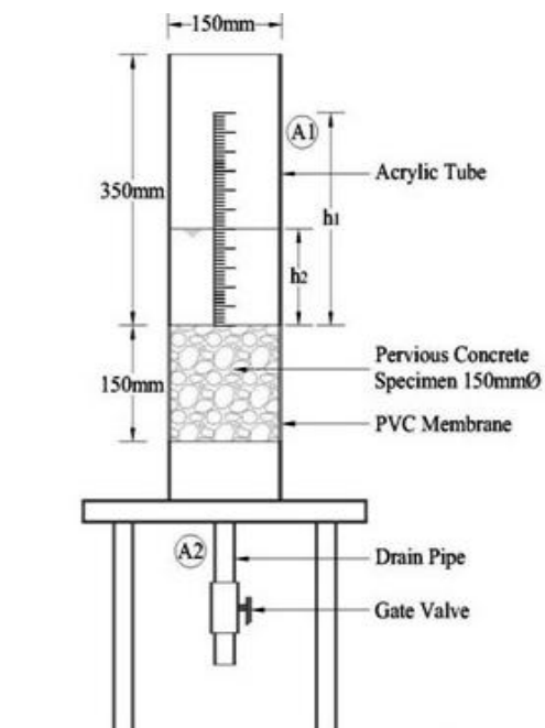
Figure 1. Falling Head Permeability Setup
