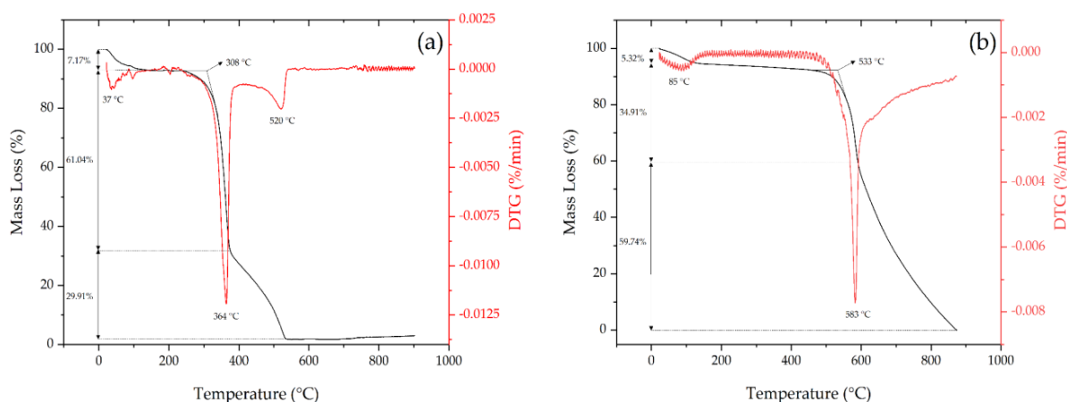
Figure 8. TGA and DTG curves obtained for (a) flax fabric; (b) aramid fabric
