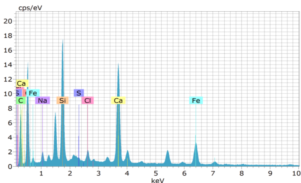
Figure 9. EDAX of M1 mix
