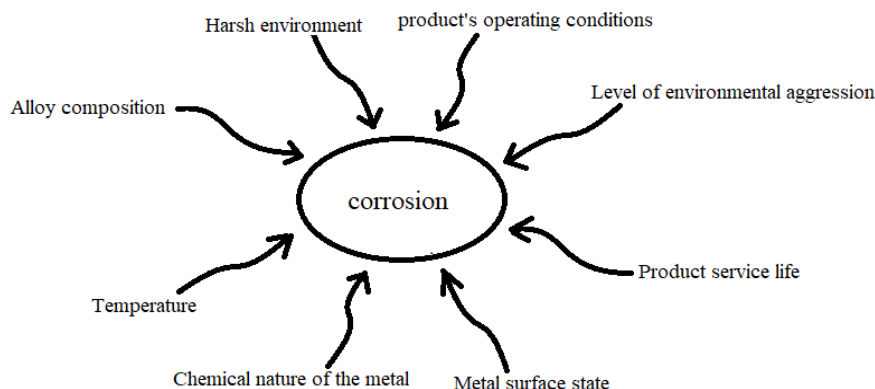
Figure 1. Some factors affecting the rate of aqueous corrosion of metallic materials
