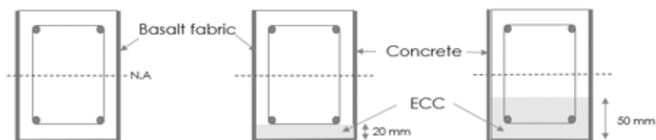
Figure 2. Details of beam
