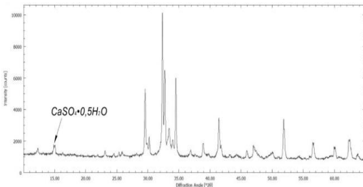
Figure 7. XRD diffractogram of cement with hemihydrate gypsum
