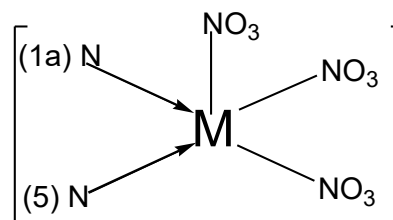
Figure 2. Metal complex (trivalent), M= Iron
