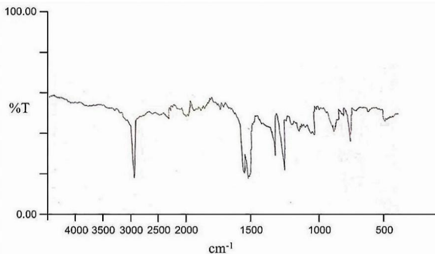
Figure 4. Infra-red spectrum of APZ
