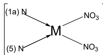
Figure 3. Metal complex (bivalent), M= Cobalt
