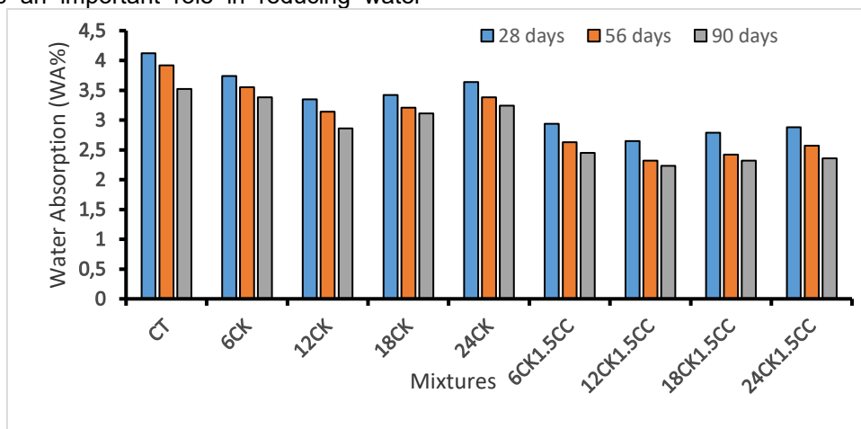
Figure 11. Water absorption of binary and ternary mixes for SCHPC incorporating CK and nano- \text{CaCO}_3 at various ages
