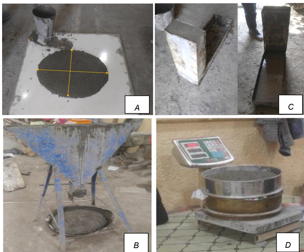
Figure 2. Fresh test procedures
