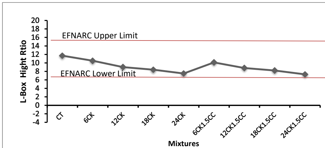
Figure 7. Segregation resistance test results
