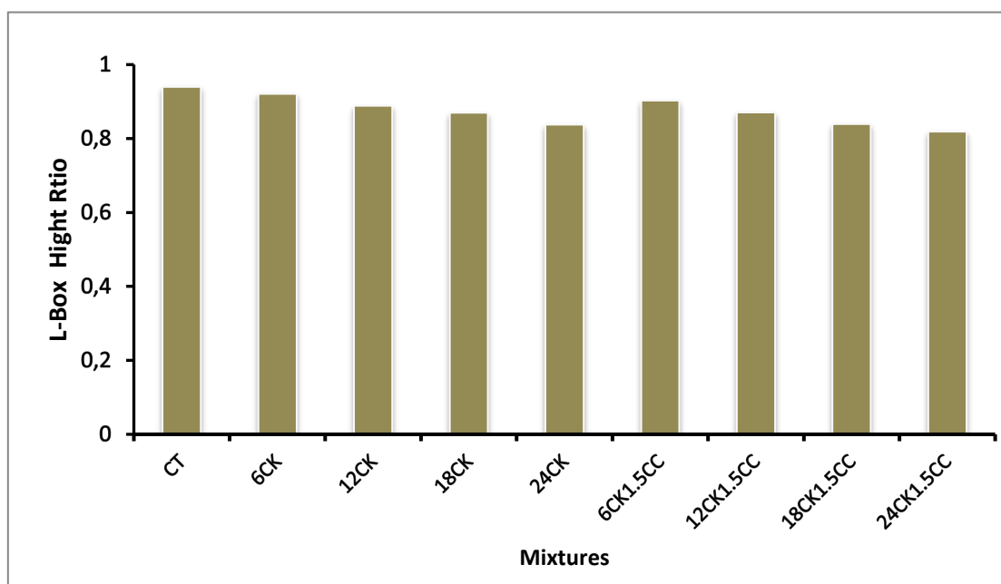
Figure 6. L-Box test results
