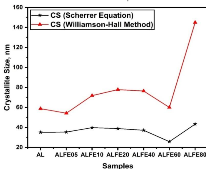
Figure 6. Comparison of Crystallite Size of \text{Al}_2\text{O}_3 - \text{Fe}_2\text{O}_3 Samples Using the Scherrer Equation and Williamson-Hall Analysis
