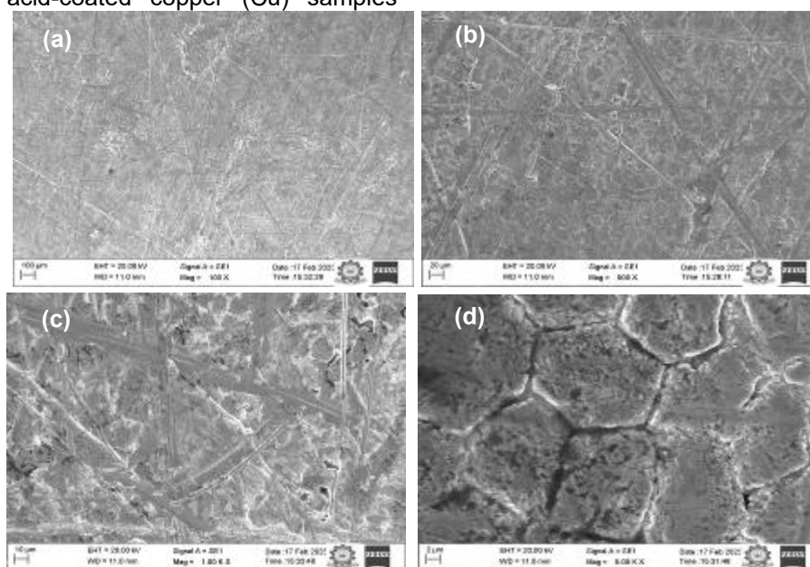
Figure 5. SEM Analysis of Uncoated Cu
