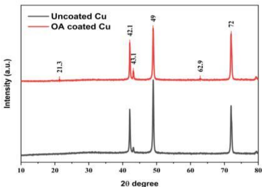
Figure 4. XRD Analysis of Uncoated and Octadecanoic Acid-Coated Copper (Cu) Samples
