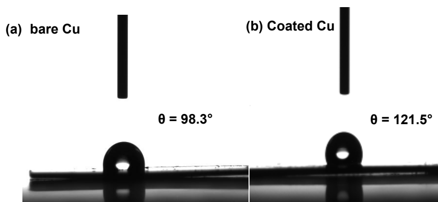
Figure 8. Contact angle measurements of (a) Bare Cu, (b) Coated Cu
