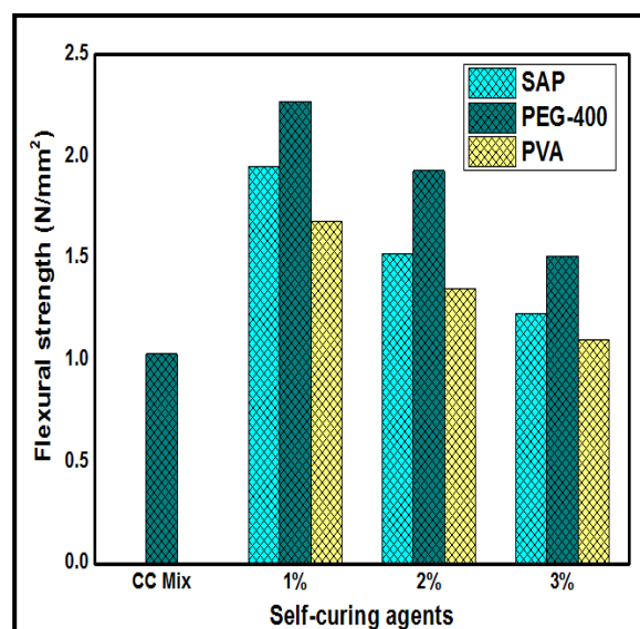
Figure 7. Test results of flexural strength of conventional and self-curing concretes
