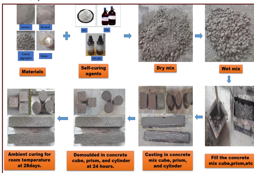
Figure 2. Mixing and Casting of Specimens
