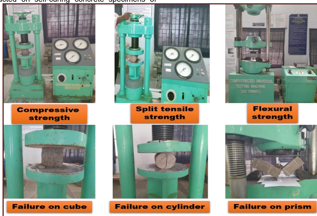
Figure 3. Experimental testing on specimens
