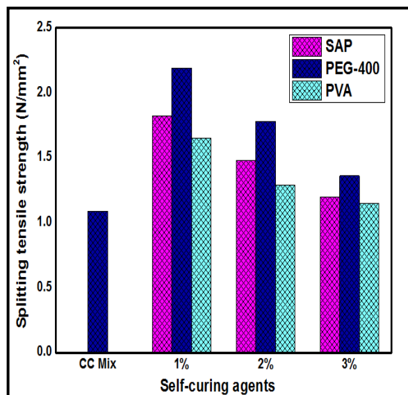
Figure 6. Test results of splitting tensile strength of conventional and self-curing concretes
