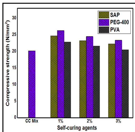
Figure 5. Test results of compressive strength of conventional and self-curing concretes
