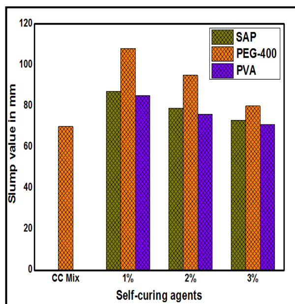
Figure 4. Test results of Slump test of conventional and self-curing concretes
