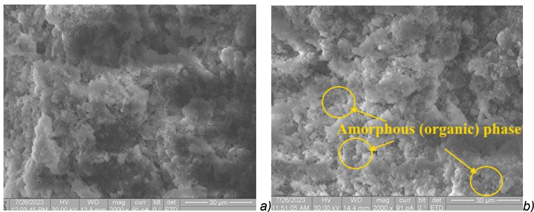
Figure 2. Structure of Lime Hardened Paste: (a) Control composition (lime + water); (b) Composition with AtrenCemHV (0.5%)
