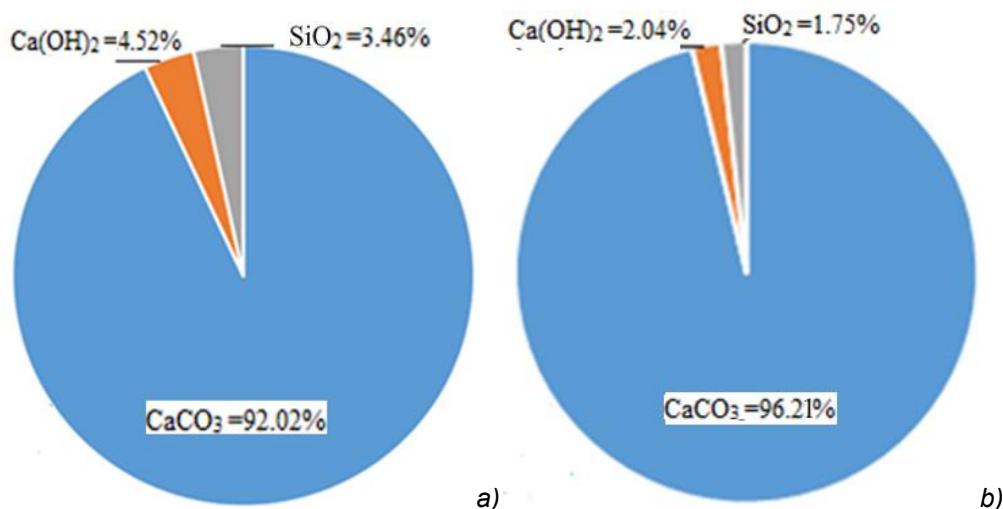
Figure 7. Mineral Content: (a) Control sample (lime) (b) Lime + 1 wt. % AtrenCemHV
