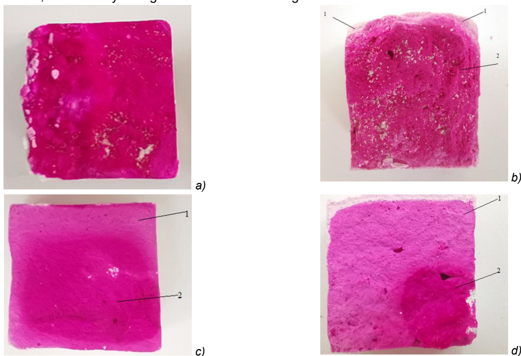
Figure 6. Carbonized Layer Changes in Lime Samples at 4 (a, b) and 10 (c, d) Days: (a, c) Control composition; (b, d) Composition with 1 wt. % AtrenCemLV; 1 - the carbonated part is indicated in light color; 2 - the low-carbonated part is indicated in dark color
