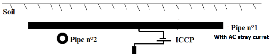
Figure 5. Schematic representation of the system employed to assess the influence of combined AC and DC stray currents on cathodic protection performance
