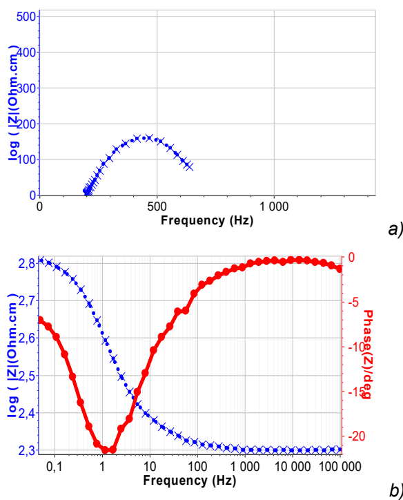
Figure 11. Nyquist plots (a) and Bode plots (b) of X70 steel in simulated soil solutions under a current density of 200 A/m 2
