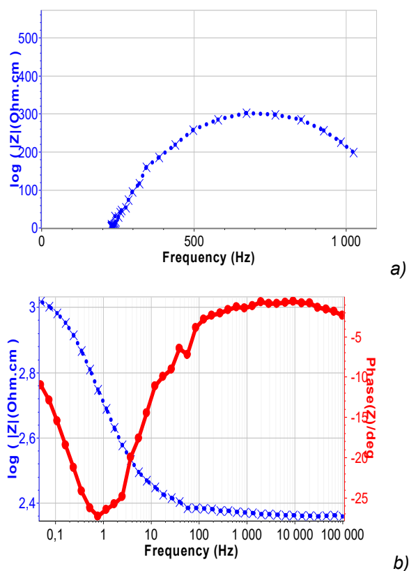
Figure 9. Nyquist plots (a) and Bode plots (b) of X70 steel in simulated soil solutions
