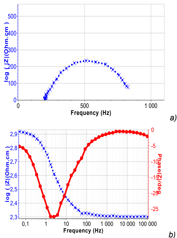
Figure 10. Nyquist plots (a) and Bode plots (b) of X70 steel in simulated soil solutions under a current density of 100 A/m 2
