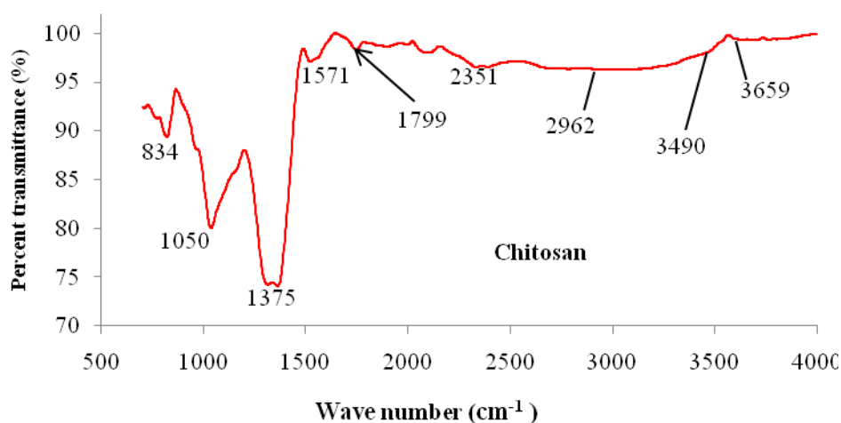
Figure 4. Fourier transformed-infrared spectrum of snail shell-chitosan
