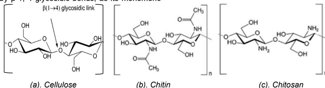
Figure 1. Chemical structure of cellulose [10], chitin (completely acetylated chitin) [11,12]; and chitosan (completely deacetylated chitosan) [13]
