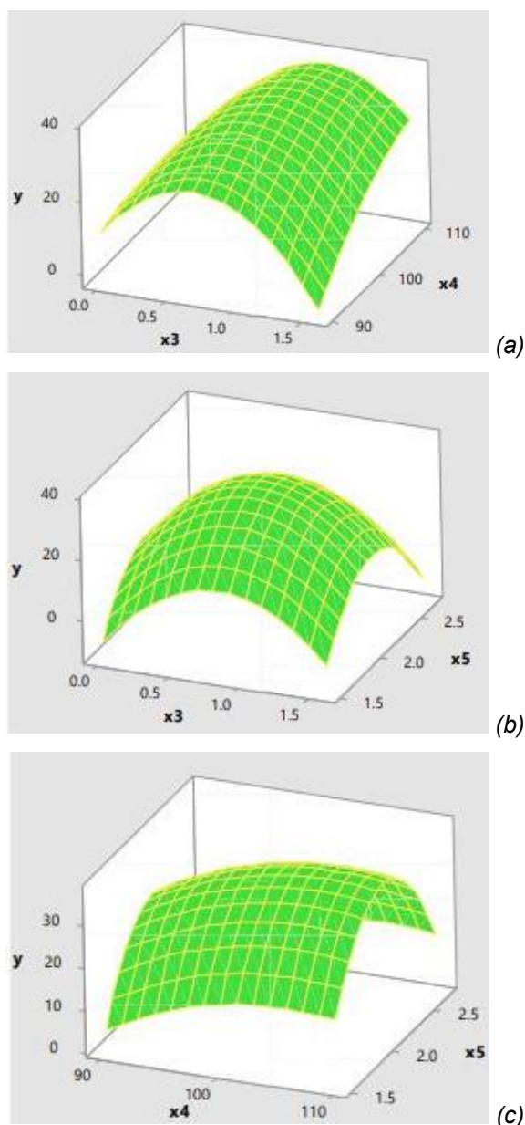
Figure 6. The 3D surface plots of the dye uptake for (a) mordant amount and dyeing temperature, (b) mordant amount and pH, (c) dyeing temperature and pH
