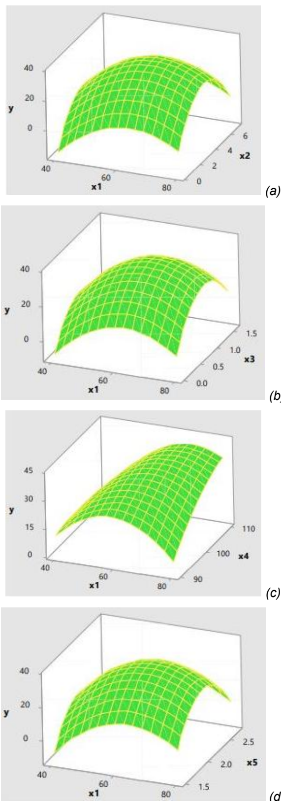
Figure 4. The 3D surface plots of the dye uptake for (a) dyeing time and dye concentration, (b) dyeing time and mordant amount, (c) dyeing time and dyeing temperature, (d) dyeing time and pH
