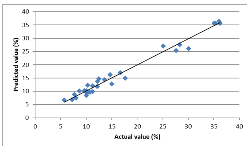
Figure 9. Experimental values versus predicted values for dye uptake for wool fiber dyed with extract of saffron petals
