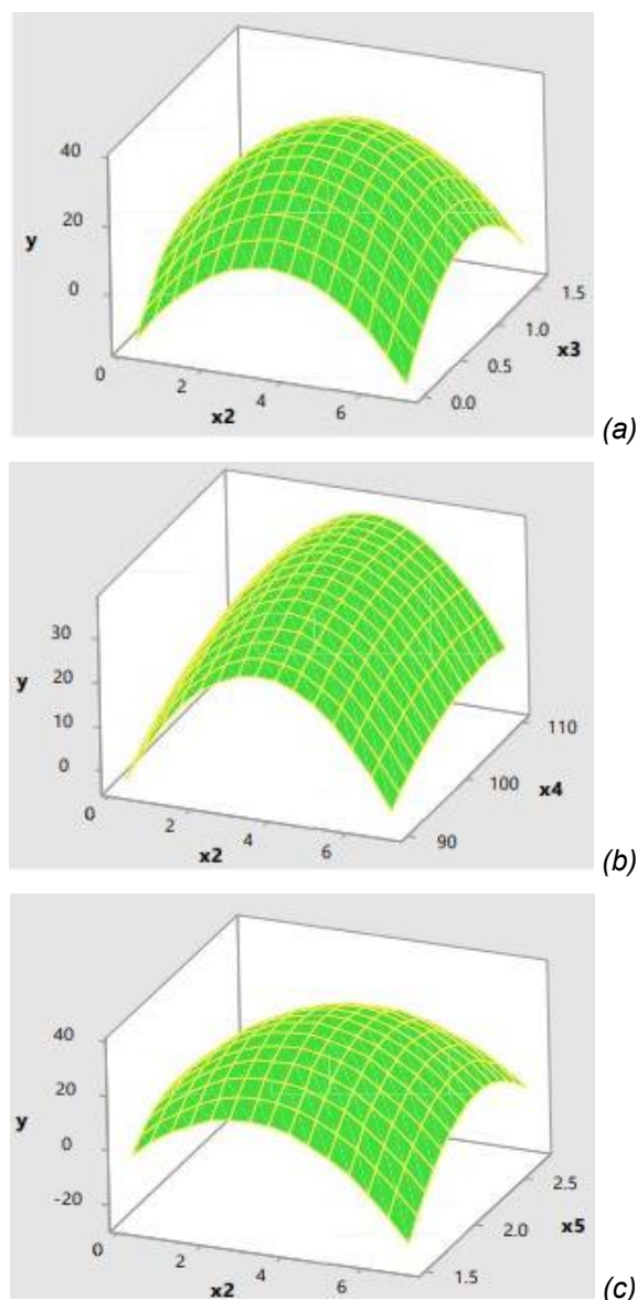
Figure 5. The 3D surface plots of the dye uptake for (a) dye concentration and mordant amount, (b) dye concentration and dyeing temperature, (c) dye concentration and pH
