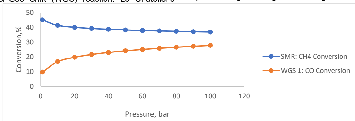
Figure 6. Effect of pressure on the methane and carbon monoxide conversions at a temperature of 1000^{\circ}\text{C} and steam to carbon (S/C=2.24) .
