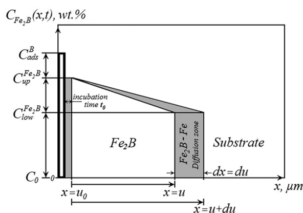
Figure 1. Boron concentration distribution across the Fe 2 B layer
