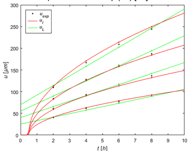
Figure 3. Predicted thicknesses of the Fe 2 B boride layer by Integral and Linear methods
