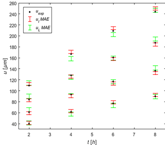
Figure 5. MAE at each predicted point for the integral and linear methods
