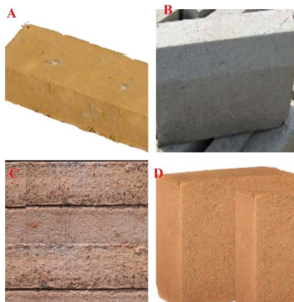
Figure 2. Agro industrial waste Bricks. A) Rice husk bricks B) Fly Ash Bricks C) Wooden dust bricks D) Coir dust bricks
