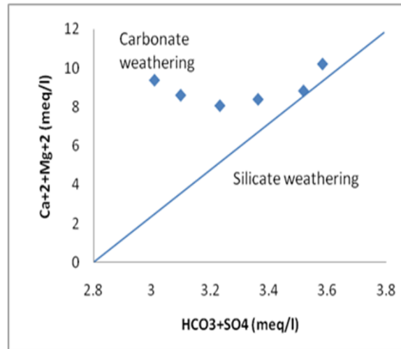
Figure 3. Scatter plot for Ca^{2+} + Mg^{2+} Vs HCO_3^- + SO_4^{2-}
