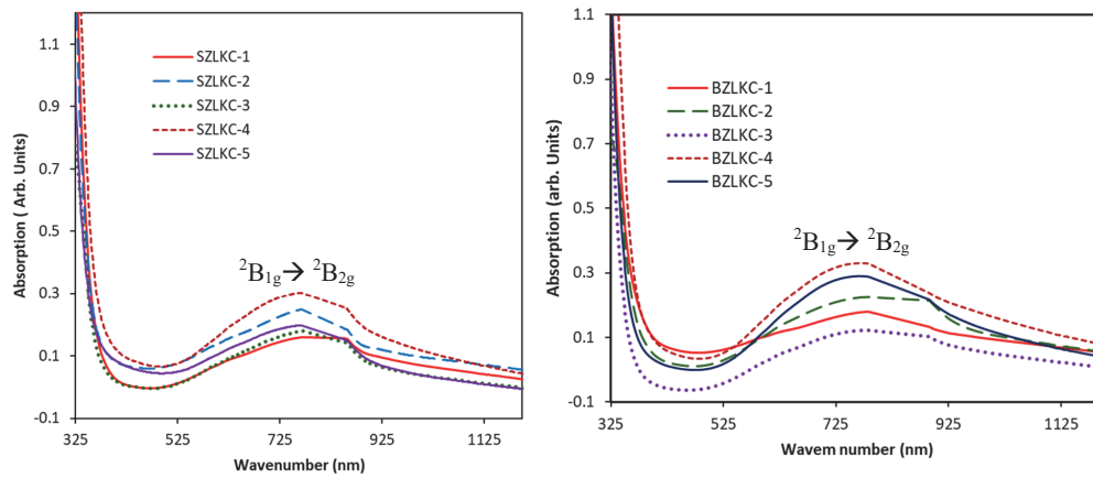
Figure 6. Optical absorption spectra of SZLK and BZLK glass systems
