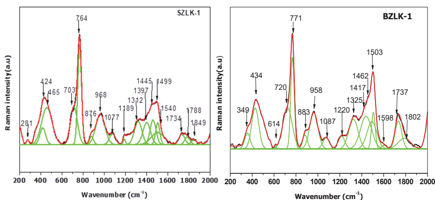
Figure 4. Deconvoluted Raman spectra of SZLK-1 and BZLK-1 glass systems
