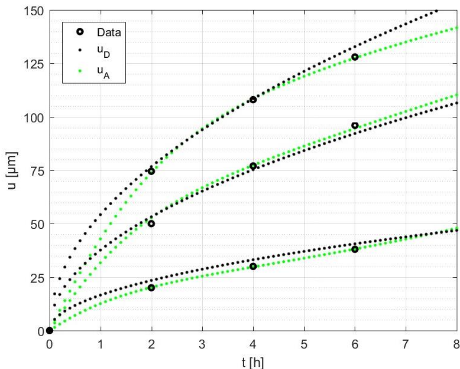
Figure 6. Simulation of the boride layer thickness over time in both models
