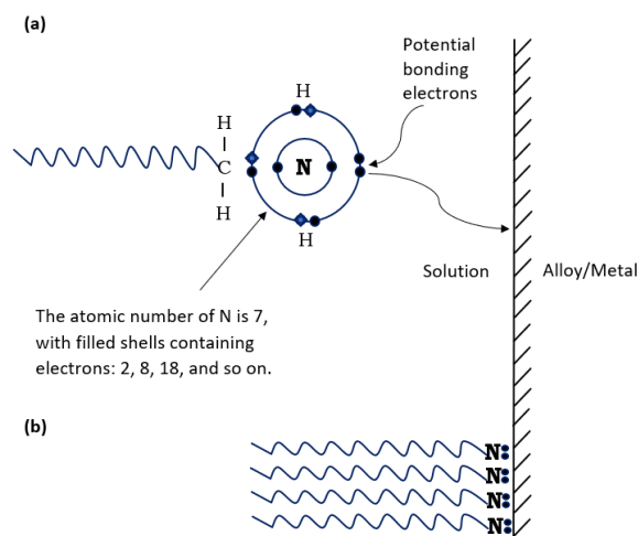
Figure 4. (a) The chemical absorption of an organic substance onto a metal surface. The symbols represent electrons from H or C atoms, whereas the solid black dots represent N atom electrons. (b) On the metal surface, a tightly packed monolayer forms [27].
