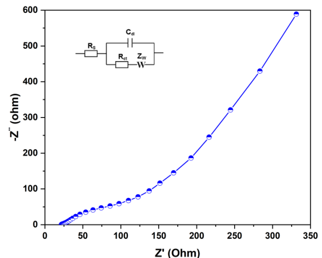
Figure 7. Nyquist plot of SnSe-PPy electrode
