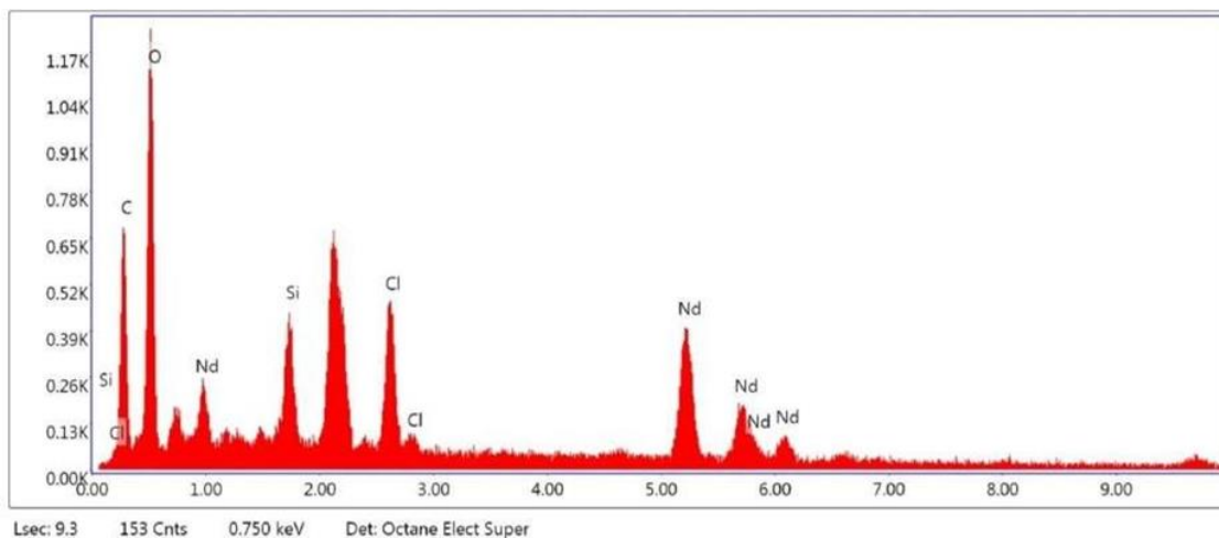
Figure 5. EDAX spectra of \text{Nd}_2\text{O}_3\text{-SiO}_2 powder sample
