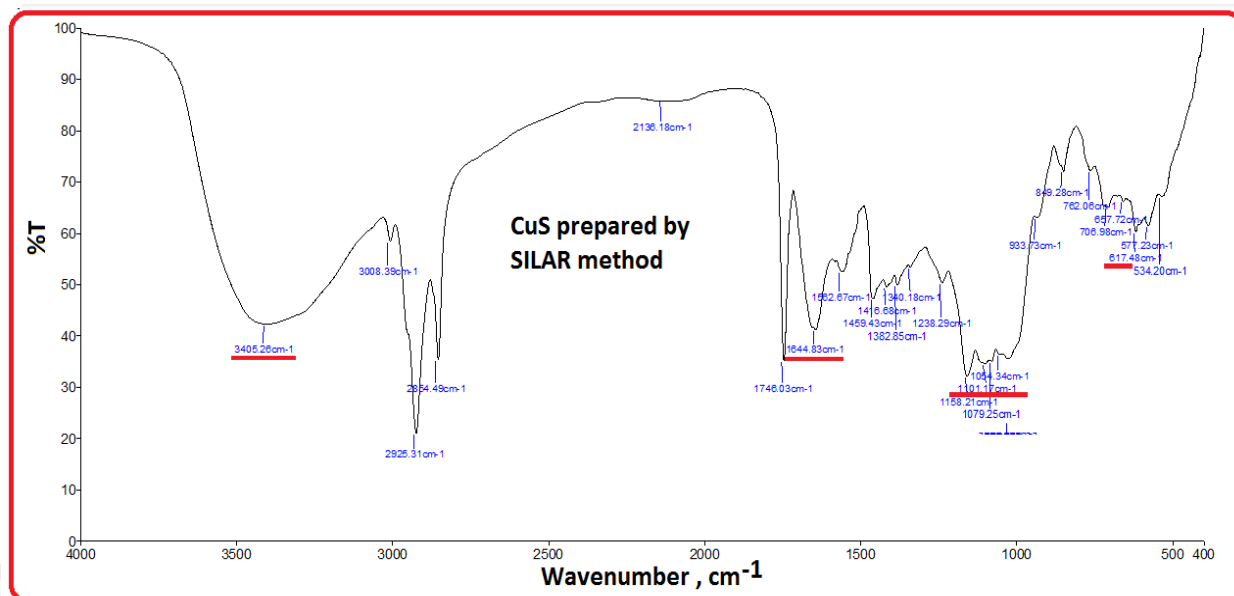
Figure 3. FTIR spectrum of copper sulphide formed on ITO glass plate by SILAR method
