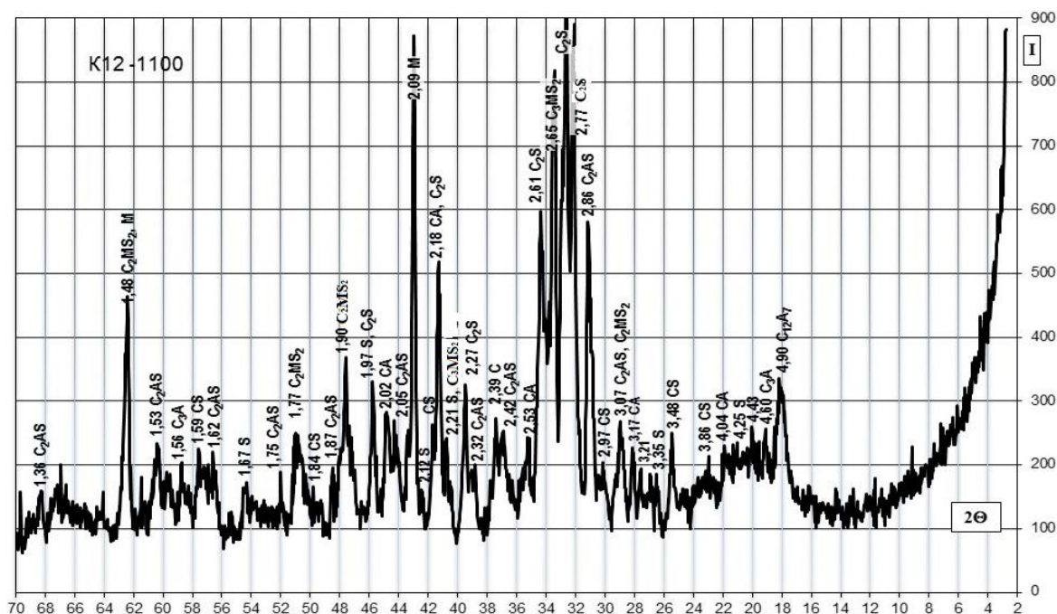
Figure 4. X-ray diffraction of sample K12 (1100°C)
