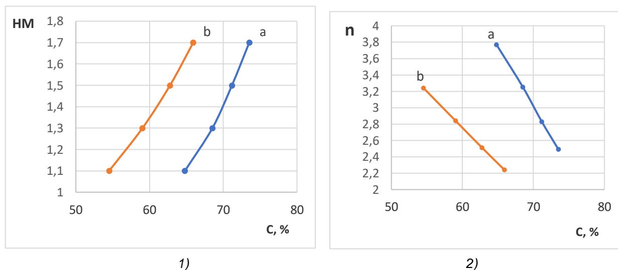
Figure 2. Dependence of the hydraulic (1) and silica (2) moduli on the concentration of the carbonate component when using pyloquartz (a) and microtalc (b)
