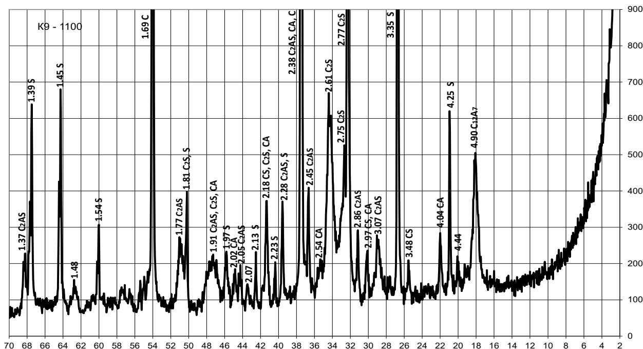
Figure 3. X-ray diffraction of sample K9 (1100°C)
