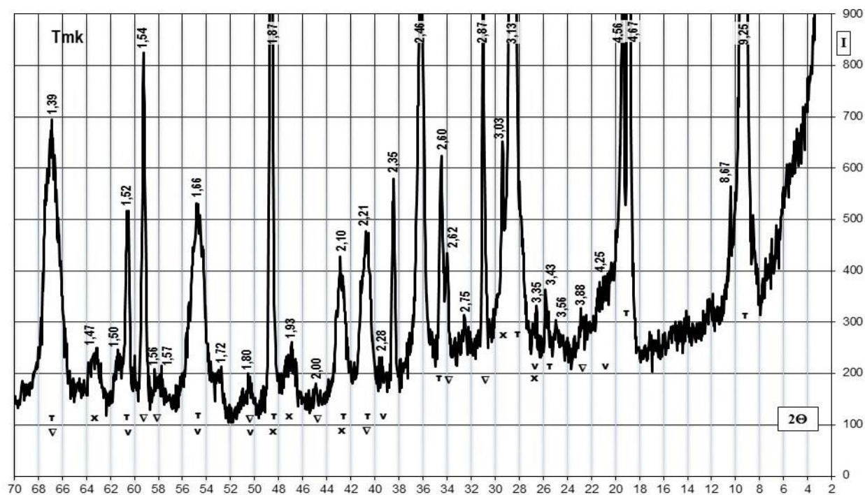
Figure 1. X-ray diffraction of microtalc: m - talc, v - \beta -quartz
