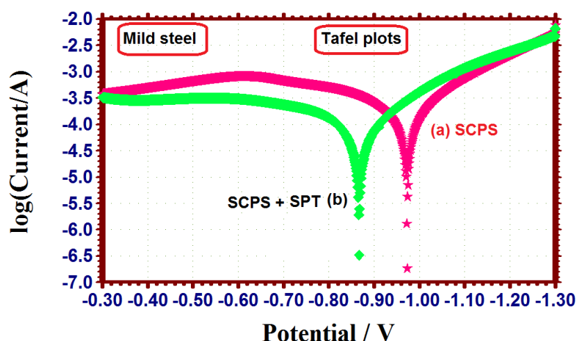
Figure 2. Potentiodynamic polarization curves of mild steel immersed in various test solutions: (a) SCPS, (b) SCPS + SPT
