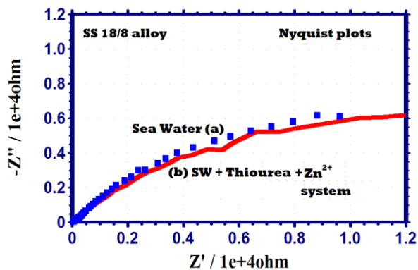
Figure 14. Nyquist plots Slika 14. Nyquist krive
