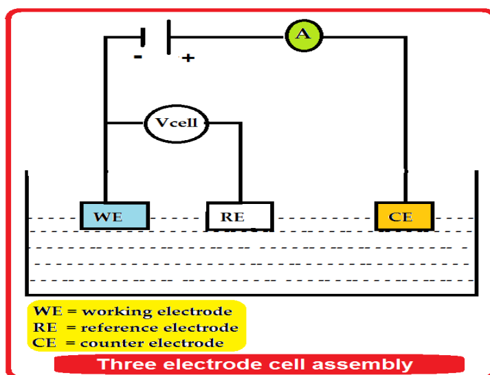
Figure 2. Three electrode cell assembly
