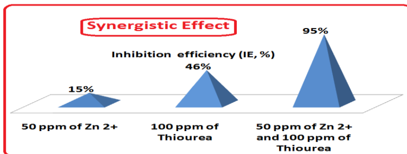
Figure 4. Synergistic effect existing between Thiourea and Zn 2+
