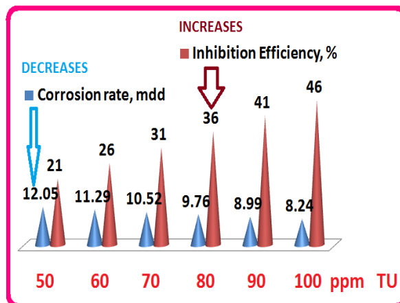
Figure 3. Correlation among concentration of Thiourea (TU), Corrosion Rate (CR, mdd) and Inhibition Efficiency (IE, %)
