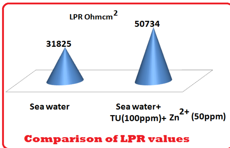
Figure 11. Comparison of LPR values between Thiourea and Zn 2+
