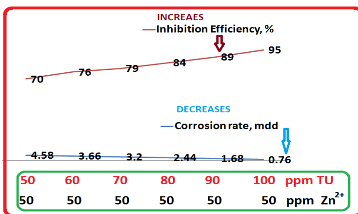
Figure 5. Inhibition efficiency and corrosion rate existing between Thiourea and Zn 2+
