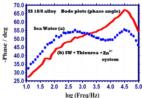
Figure 16. Bode plots (phase angle) Slika 16. Bode krive (fazni ugao)
