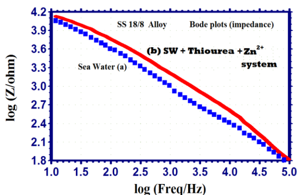
Figure 15. Bode plots (Impedance) Slika 15. Bode krive (impedansa)
