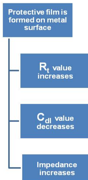
Figure12. Correlation among various AC impedance parameters
