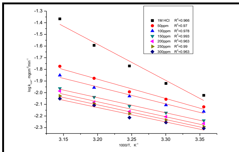
Figure 8. Log k (corrosion rate) – 1/T curves for mild steel in 1 M HCl in the absence and presence of different doses of Tilia Leaves extract
