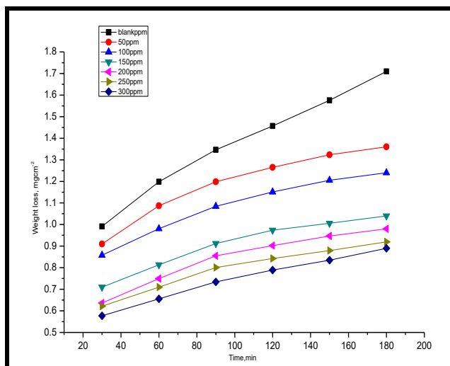
Figure 1. Weight loss-time curves for the corrosion of mild steel in 1 M HCl in the absence and presence of different doses of Tilia Leaves at 25°C
