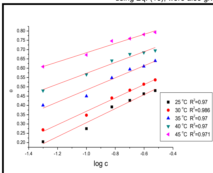
Figure 7. Temkin adsorption plots for mild steel in 1M HCl containing various doses of Tilia Leaves at 25°C
