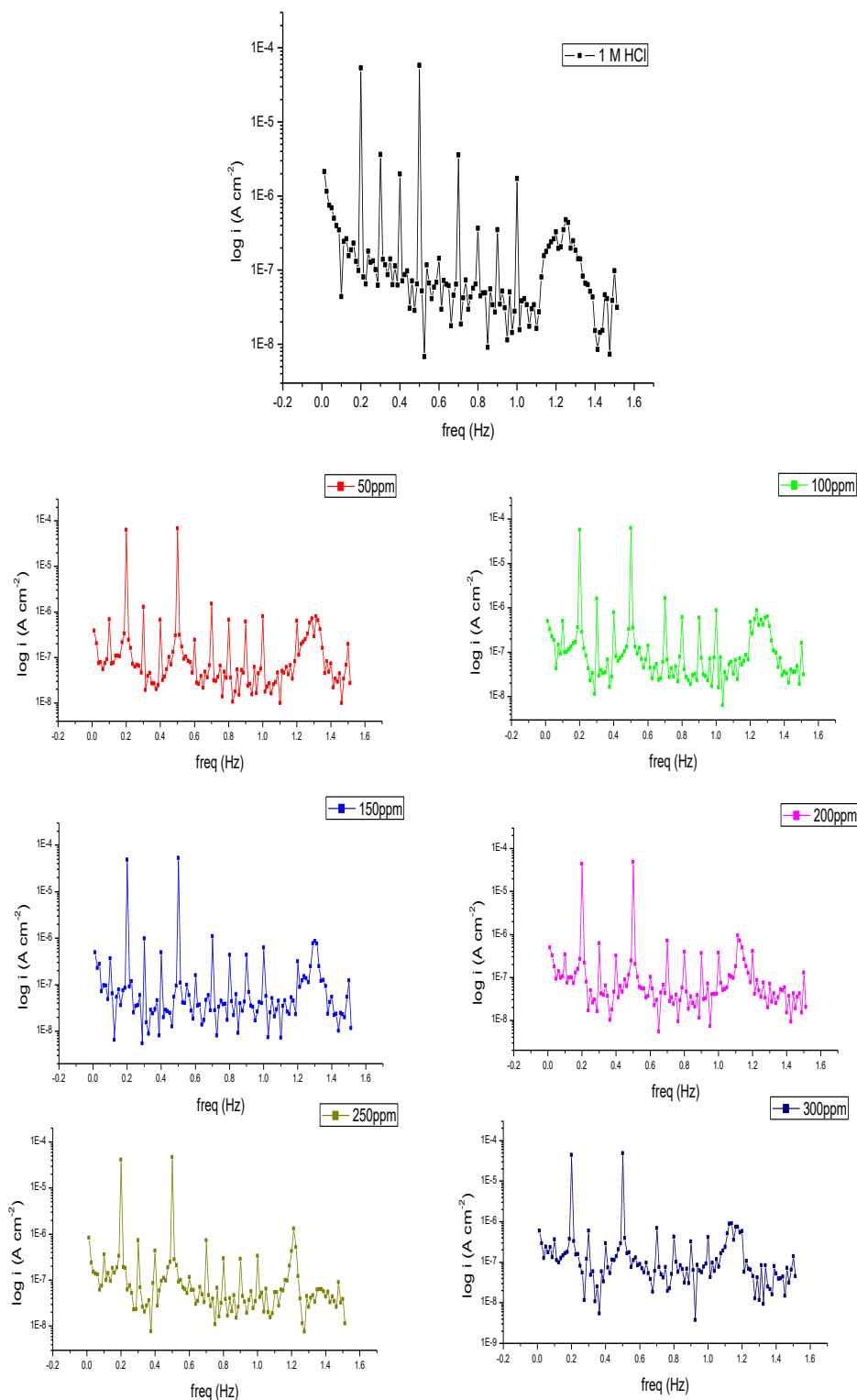
Figure 6. Intermodulation spectrums for the corrosion of mild steel in 1M HCl without and with various doses of Tilia Leaves at 25°C
