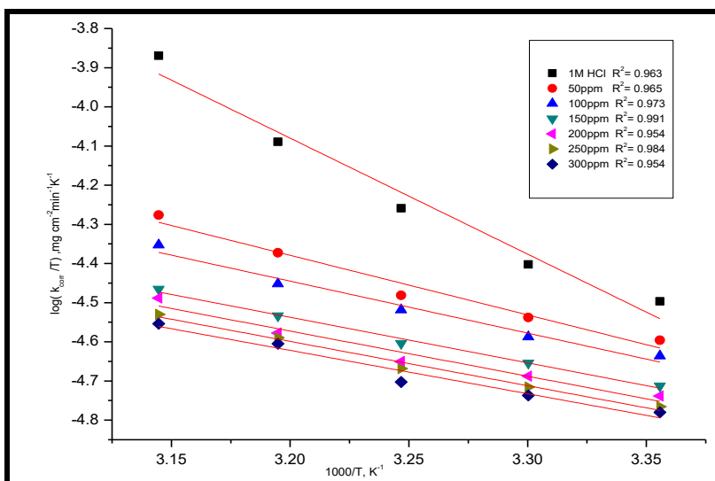
Figure 9. Log k (corrosion rate)/T – 1/T curves for mild steel in 1 M HCl in the absence and presence of different doses of Tilia Leaves extract
