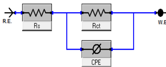
Figure 3. Electrical equivalent circuit used to fit the impedance data
