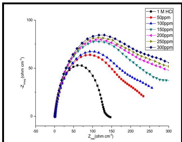
Figure 2. Nyquist plots for mild steel in 1M HCl at different doses of Tilia Leaves
