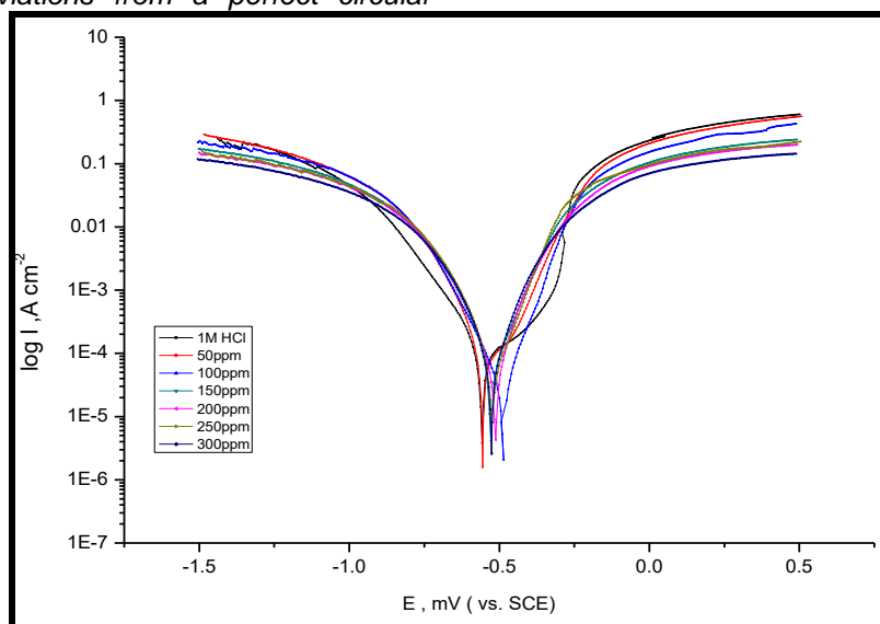
Figure 5. Potentiodynamic plots for corrosion of mild steel in 1 M HCl in the absence and presence of different doses of Tilia Leafs at 25°C
