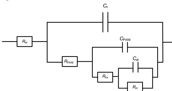
Figure 8 - Electrical equivalent circuit for steel with polyaniline powder dispersed in polymer binder and epoxy top coat, in 3\% \text{ NaCl} .
