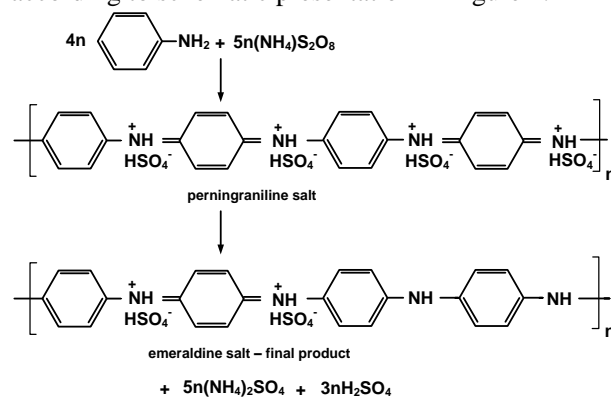
Figure 4 - Chemical synthesis of polyaniline
