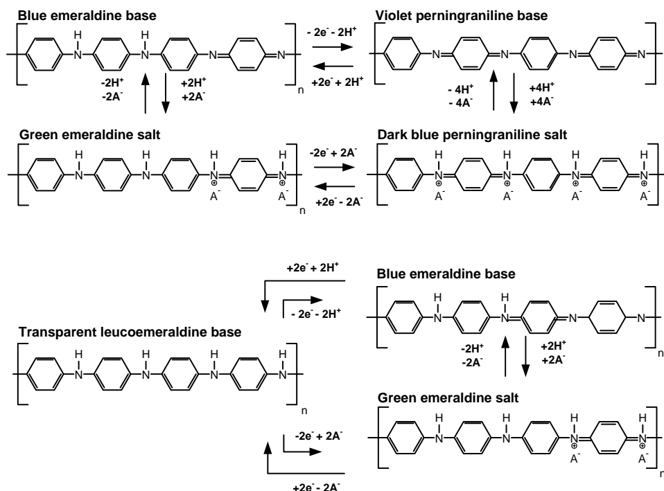
Figure 3 - Different forms of polyaniline, and its mutual conversions.
