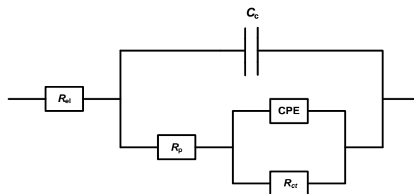
Figure 6 - Common electrical equivalent circuit used to fit EIS data for organic coatings.
