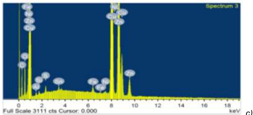
Figure 14 - EDX spectra of alpha brass (c) After 24 h of immersion in 0.5 M \text{HNO}_3 + 300 ppm Augmentin
