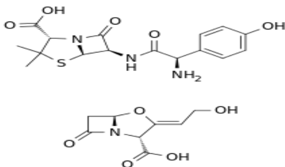
(2 S ,5 R ,6 R )-6-[[[(2 R )-2-amino-2-(4-hydroxyphenyl)acetyl]amino]-3,3-dimethyl-7-oxo-4-thia-1-azabicyclo[3.2.0]heptane-2-carboxylic acid;(2 R ,3 Z ,5 R )-3-(2-hydroxyethylidene)-7-oxo-4-oxa-1-azabicyclo[3.2.0]heptane-2-carboxylic acid.
