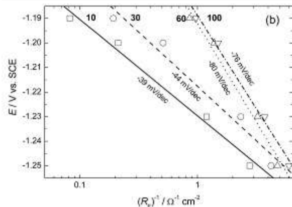
Figure 5 - (a) C_{dl} vs. E dependences. (b) E vs. \log (R_F)^{-1} dependences.
