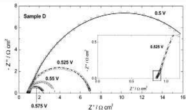
Figure 6 - Nyquist plots for the OER at sample D recorded at different potentials (marked in the figure): Inset – high frequency end showing small semi-circle marked with square.
