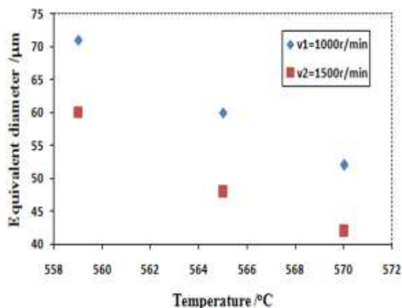
Figure 2 - Equivalent diameters of Si particles versus temperature
