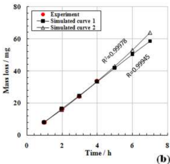
Figure 5 - Mass loss versus time: 1-Linear equation 2- Quadratic equation for sample a) A; b) D
