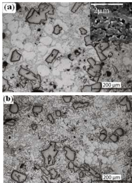
Figure 1 - Microstructures of samples a) A, b) D (OM, polished)
