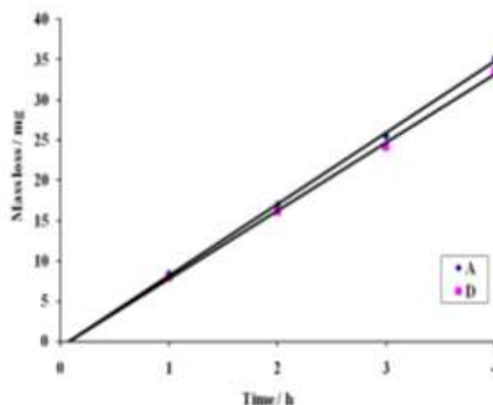
Figure 4 - Cavitation erosion of tested samples as a function of time
