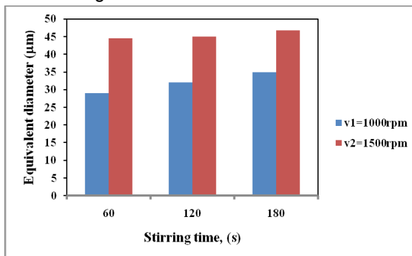
Fig. 3 - Average particle size of primary silicon of rheocast samples
