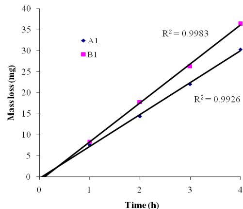
Fig.4 - Cavitation erosion of tested samples as a function time
