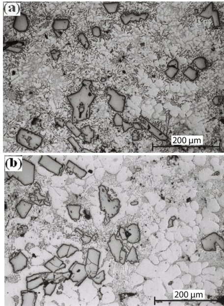
Fig.2 - Distribution of Si particles: a) stirring speed 1000rpm, after 60s; b) stirring speed 1500rpm, after 60s
