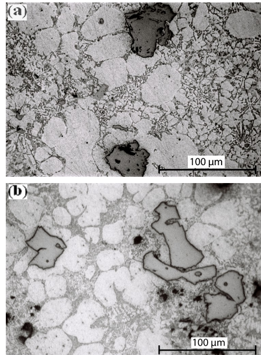
Fig.1 - Microstructure of Al18wt%Si alloy: a) stirring speed 1000rpm, after 60s; b) stirring speed 1500rpm, after 60s
