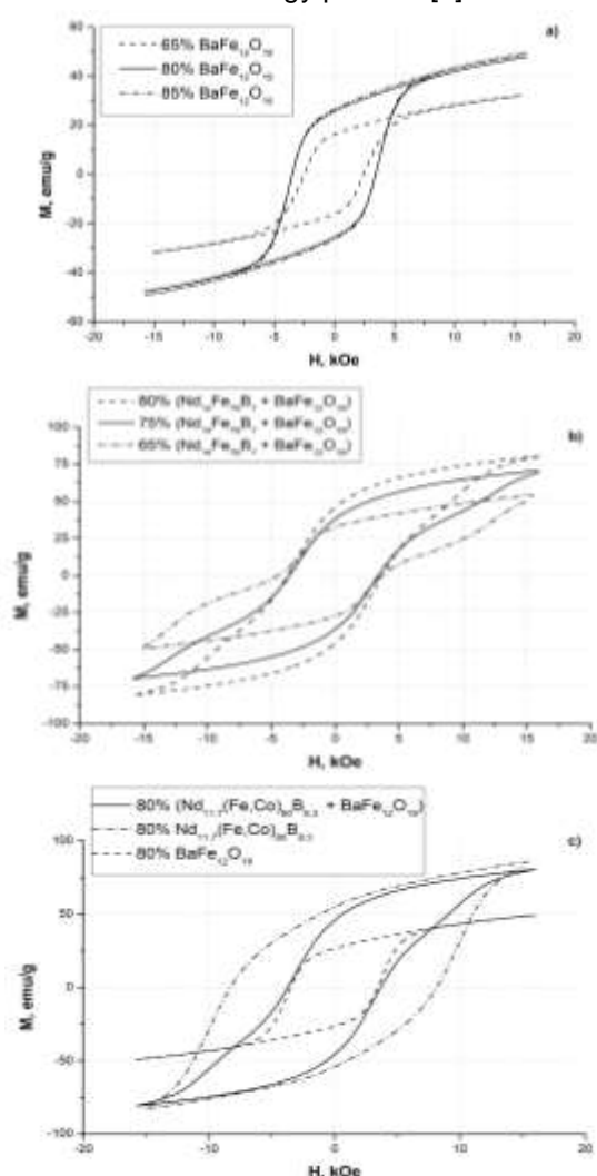
Figure 2. VSM hysteresis loops for different types of polymer bonded composites
