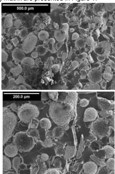
Figure 1 - SEM micrographs of Nd-Fe-B/barium-ferrite/epoxy composites
